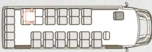
PASSENGERS SEATS-Typical Lay-out: 29 + 1 (Hostess)
