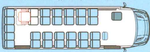
PASSENGERS SEATS-Typical Lay-out: 31+(1)
